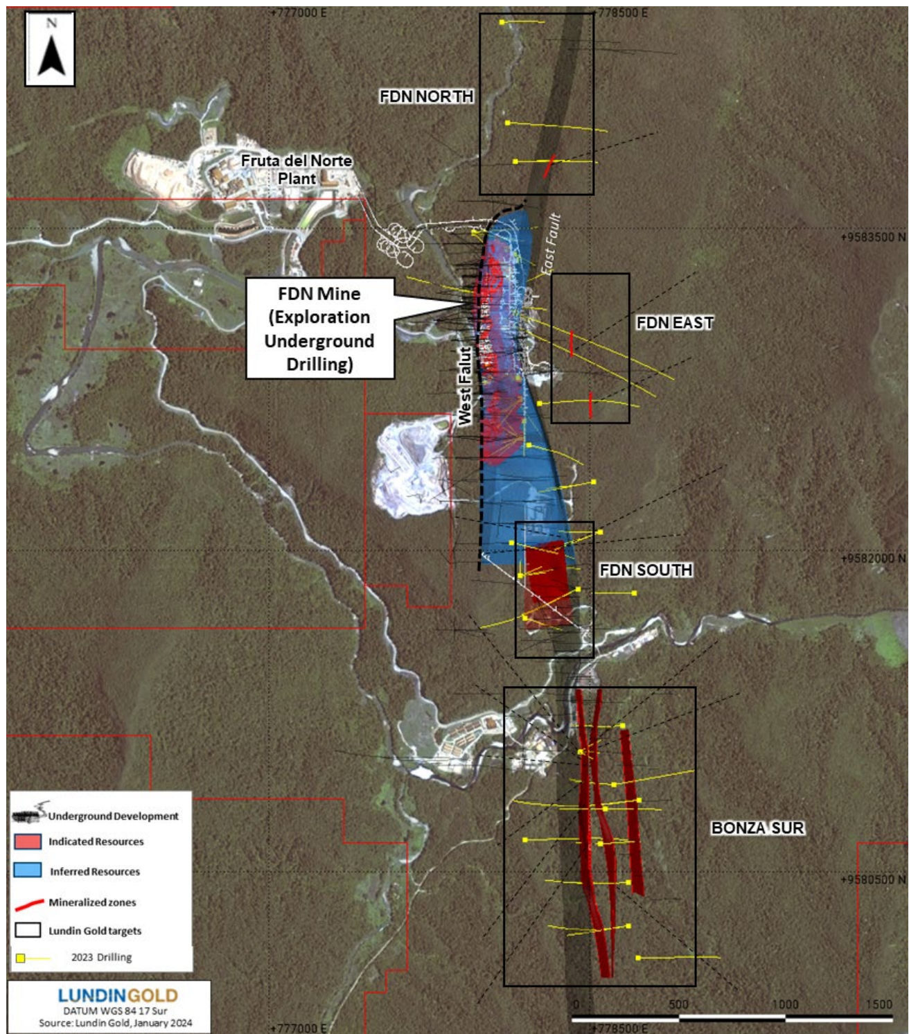
Figure 2: Drilling program location at La Zarza Concession (Near Mine)
